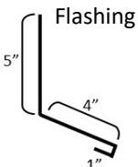
Apron or Side Wall Flashing
